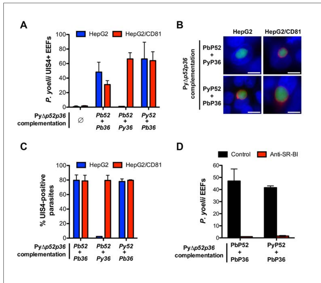
Figure 7. Transgenic P. yoelii sporozoites expressing PbP36 can infect CD81-null cells via SR-BI. (A) HepG2 (blue) and HepG2/CD81 cells (red) were incubated with genetically complemented Py \Delta p52/p36 sporozoites, and fixed 24 hr post-infection. The number of UIS4-positive vacuoles was then determined by immunofluorescence. (B) Immunofluorescence analysis of UIS4 expression in HepG2 or HepG2/CD81 cells infected with sporozoites of Py \Delta p52/p36 parasites genetically complemented with P52 and P36 from P. berghei or P. yoelii . Cells were fixed with PFA, permeabilized, and stained with anti-UIS4 antibodies (red) and the nuclear stain Hoechst 33342 (blue). Parasites were detected based on GFP expression (green). Scale bars, 10 \mu m. (C) Quantification of UIS4 expression in HepG2 (blue) and HepG2/CD81 cells (red) infected with genetically complemented Py \Delta p52/p36 sporozoites and processed as in B for immunofluorescence. (D) HepG2 cells were incubated with Py \Delta p52/p36 sporozoites complemented with PbP36 and either PbP52 or PyP52 , in the presence or absence of anti-SR-BI antibodies. Infected cultures were fixed 24 hr post-infection, and the number of EEFs was then determined by fluorescence microscopy.
